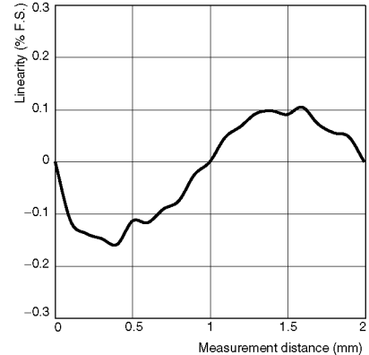
ZX-ED02T/ZX-EM02T
